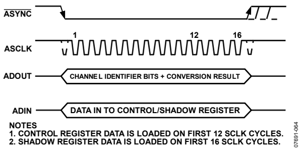
Figure 64. ADC Normal Mode Operation
