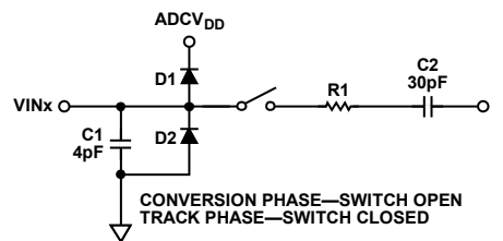
Figure 56. Equivalent Analog Input Circuit
