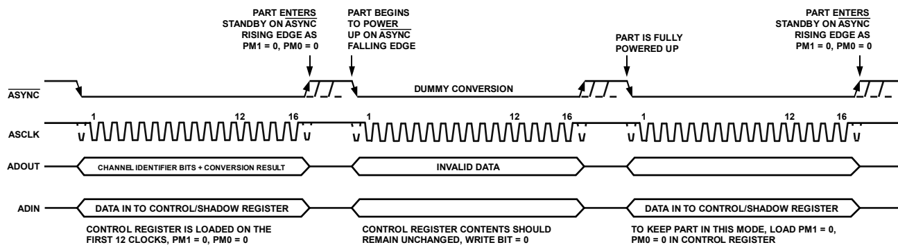
Figure 67. Autostandby Mode Operation
